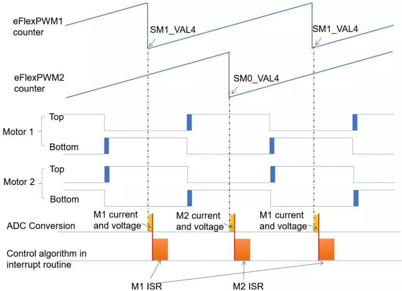
Figure 67-4. Synchronization between ADC and PWMs
