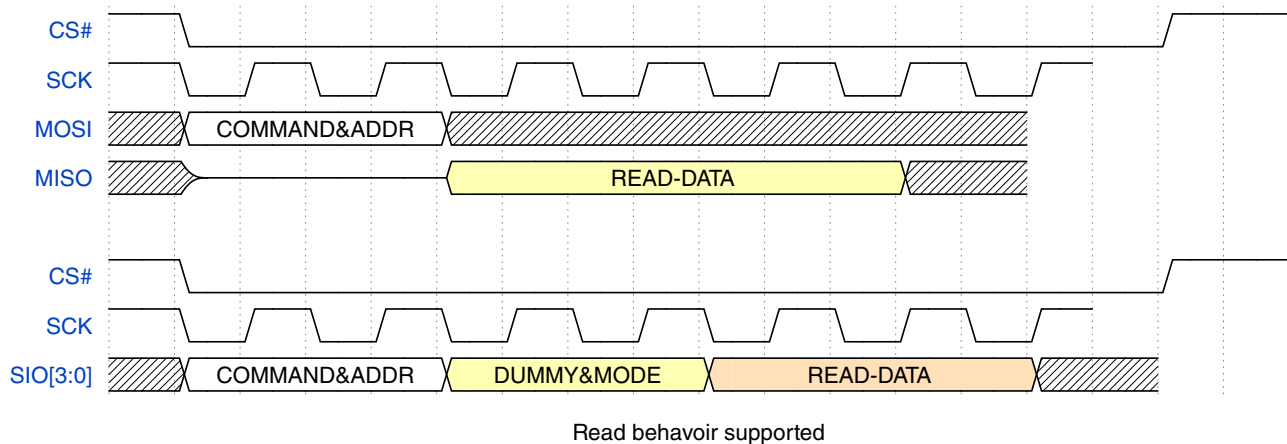
Figure 27-28. Supported Read Behavior
