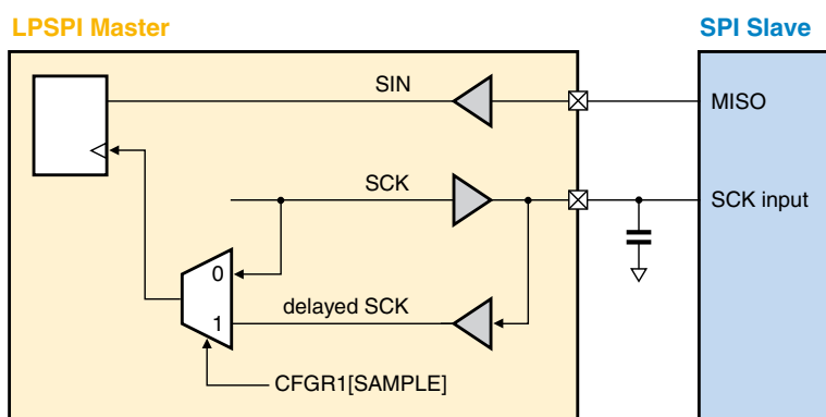
Figure 48-3. Clock loopback
