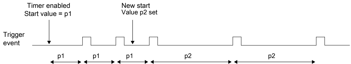
Figure 53-4. Dynamically setting a new load value
