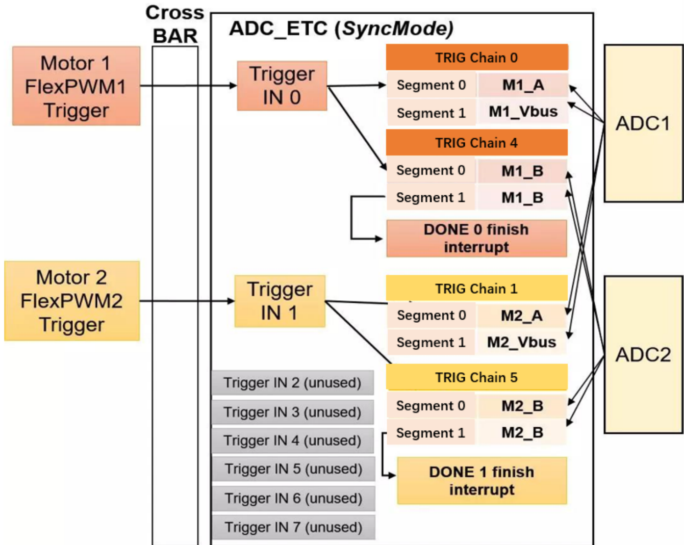
Figure 67-5. The configuration of ADC_ETC for dual motor control
