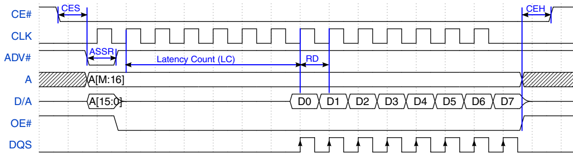
Figure 25-56. SYNC Flash Read in ADMUX Address Mode
