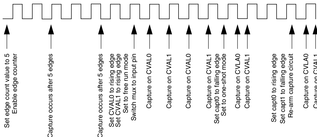
Figure 55-10. Capture Capabilities of the E-Capture Circuit
