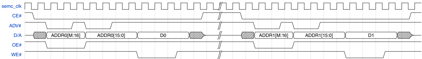
Figure 25-62. ASYNC SRAM Write in AADM Address Mode
