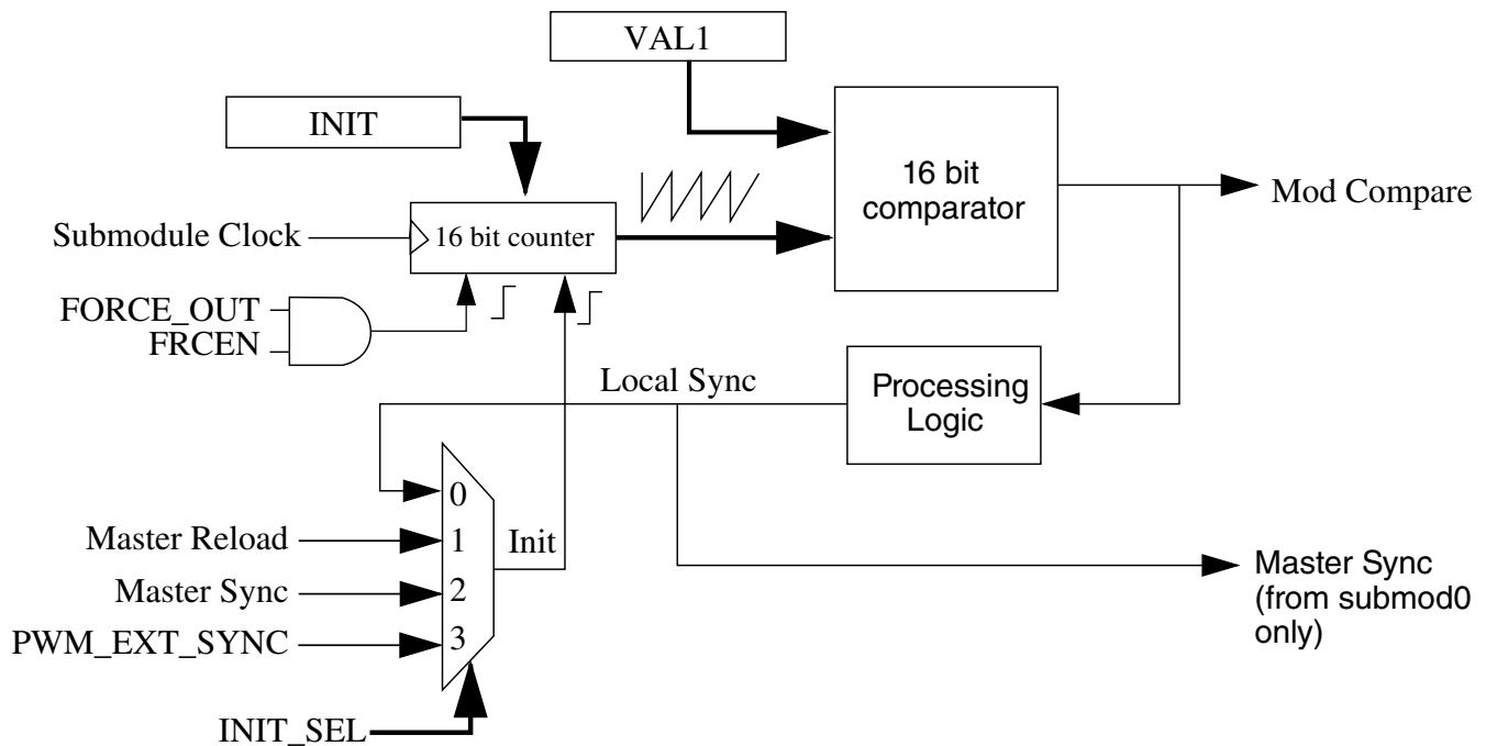
Figure 55-17. Submodule Timer Synchronization
