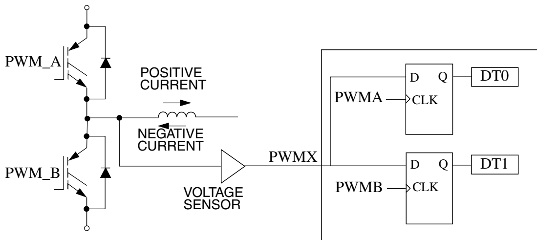
Figure 55-25. Current-status Sense Scheme for Deadtime Correction
