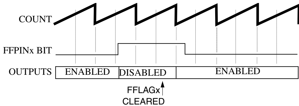
Figure 55-32. Manual Fault Clearing (FCTRL[FSAFE]=0)
