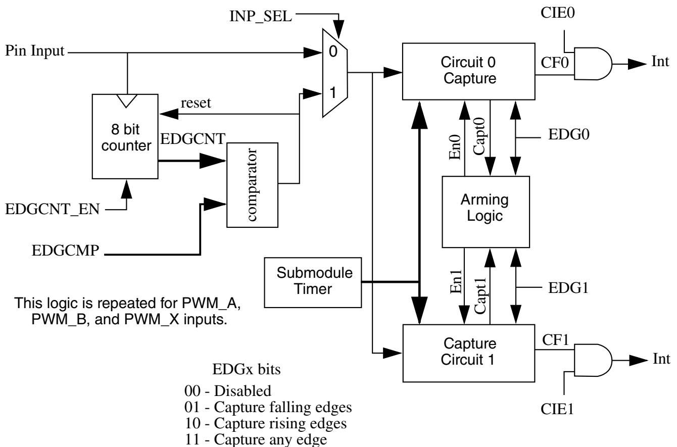
Figure 55-29. Enhanced Capture (E-Capture) Logic
