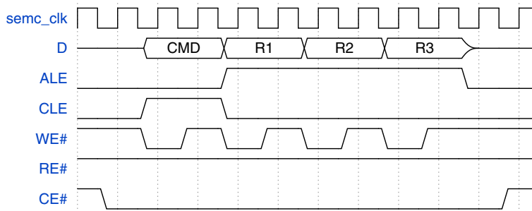
Figure 25-34. NAND Flash Access Address Type - Three Bytes Row Address
