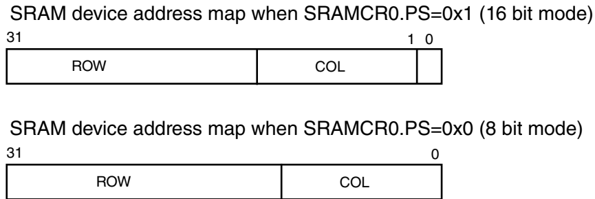
Figure 25-58. SRAM Address Multiplexing
