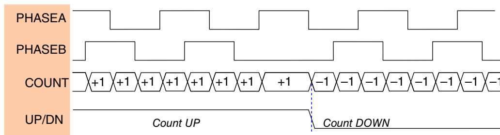
Figure 56-3. Quad Decoder Signals
