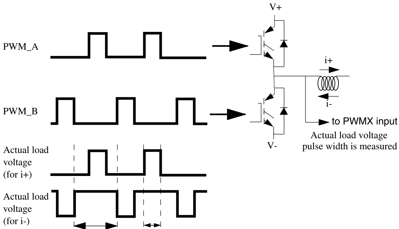
Figure 55-11. Output Pulse Width Measurement Possible with the E-Capture Circuit
