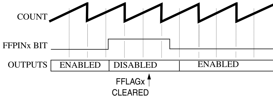
Figure 55-33. Manual Fault Clearing (FCTRL[FSAFE]=1)
