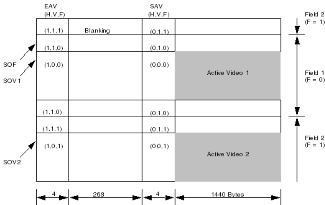
Figure 34-4. BT.656 Interlace Mode (PAL)
