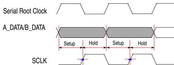
Figure 27-19. SDR instruction in SDR sequence
