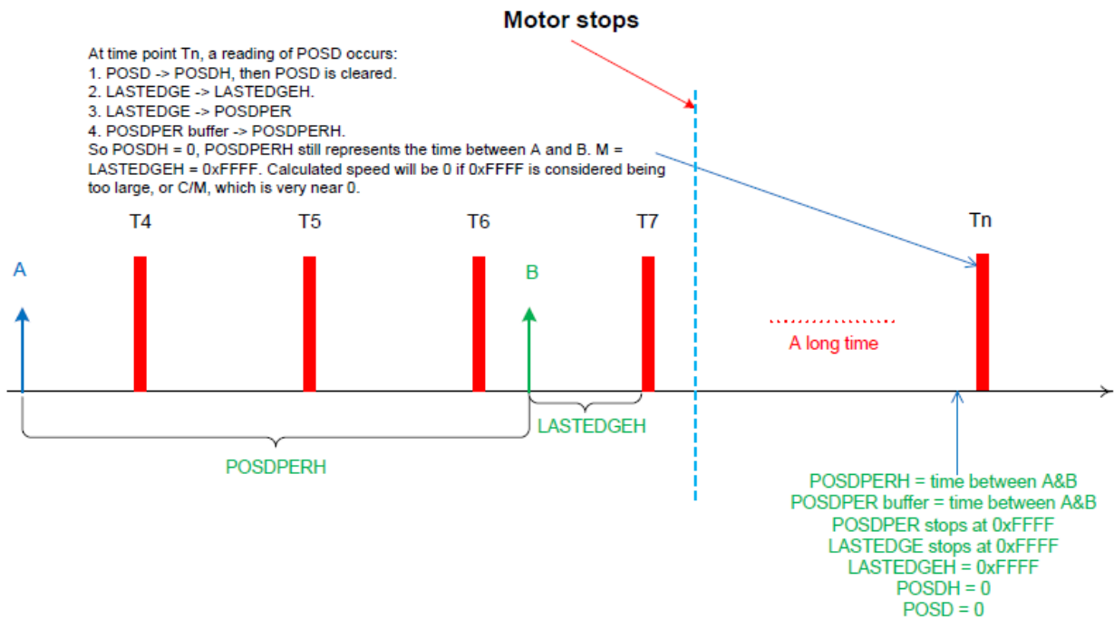
Figure 56-12. Speed measurement at time point Tn
