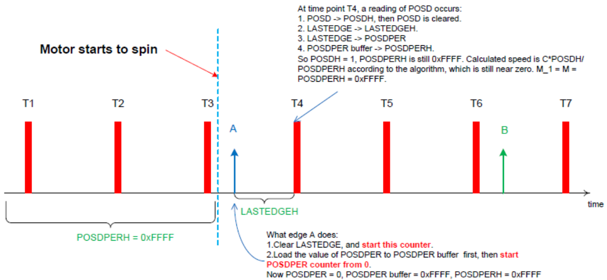
Figure 56-8. Speed measurement at time point T4
