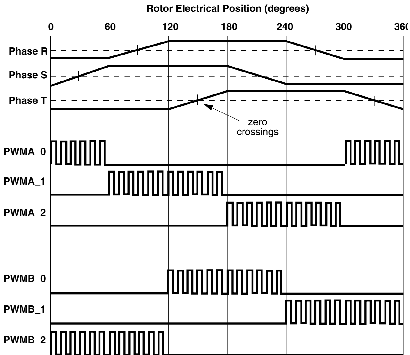
Figure 55-12. Sensorless BLDC Commutation Using the Force Out Function
