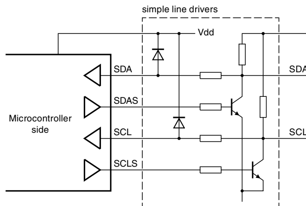
Figure 47-3. I 2 C 4-wire serial bus
