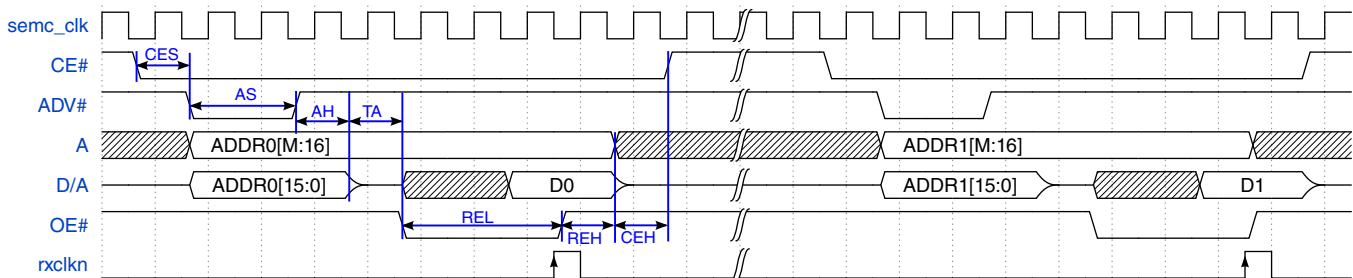
Figure 25-52. ASYNC NOR Flash Read in ADMUX Address Mode
