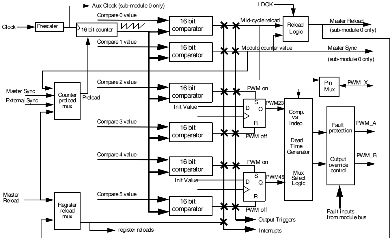
Figure 55-2. PWM Submodule Block Diagram
