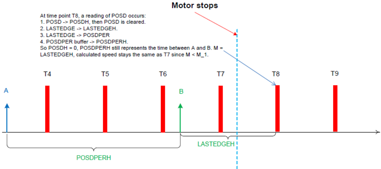
Figure 56-11. Speed measurement at time point T8
