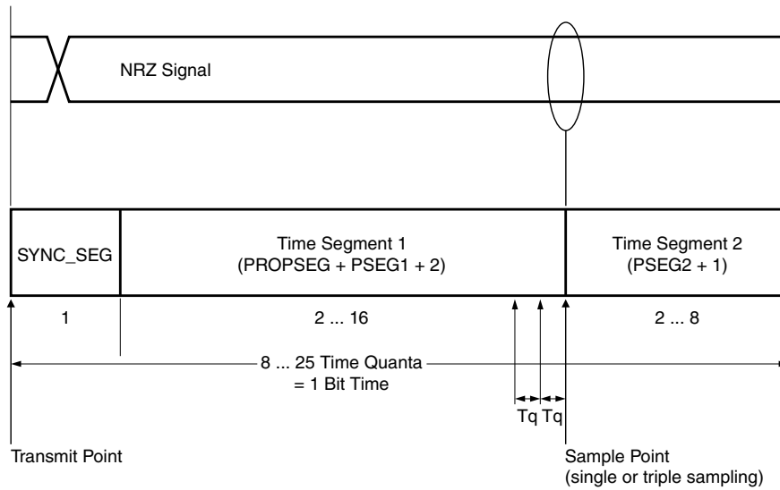
Figure 45-9. Segments within the bit time (example using CTRL1 bit timing variables for Classical CAN format)
