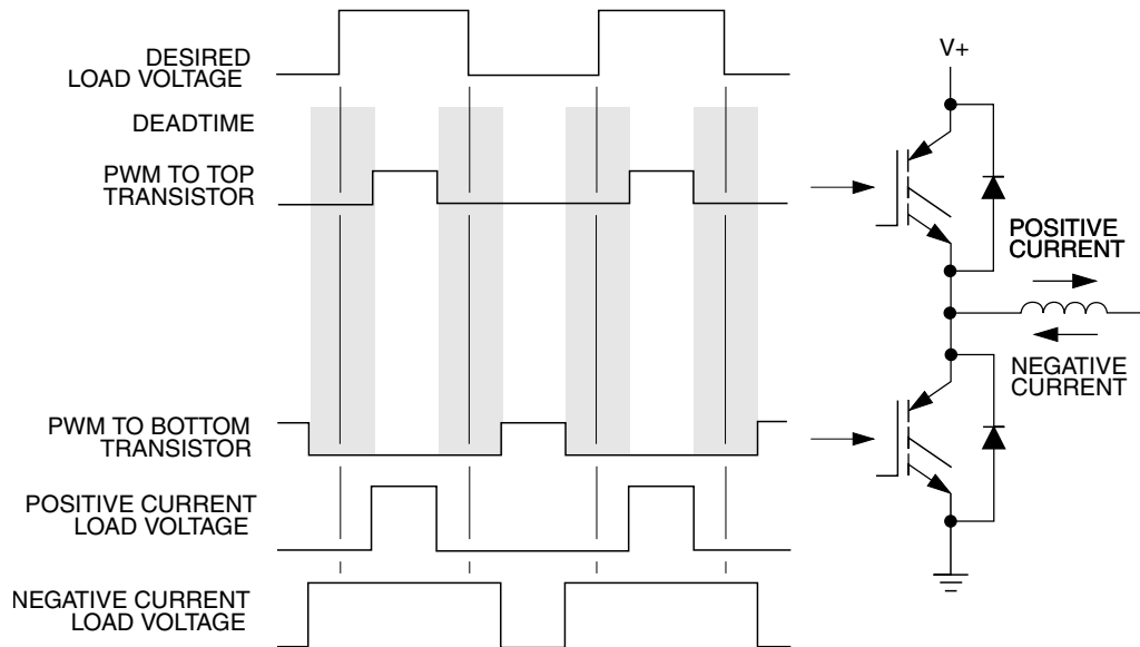
Figure 55-24. Deadtime Distortion
