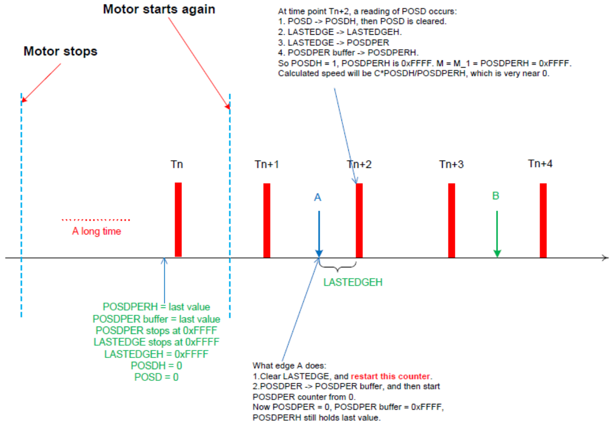
Figure 56-13. Speed measurement at time point T_{n+2}
