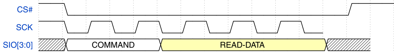
Figure 27-27. Unsupported Read Behavior
