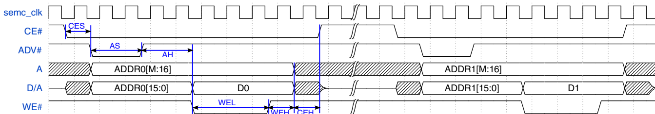
Figure 25-54. ASYNC NOR Flash Write in ADMUX Address Mode
