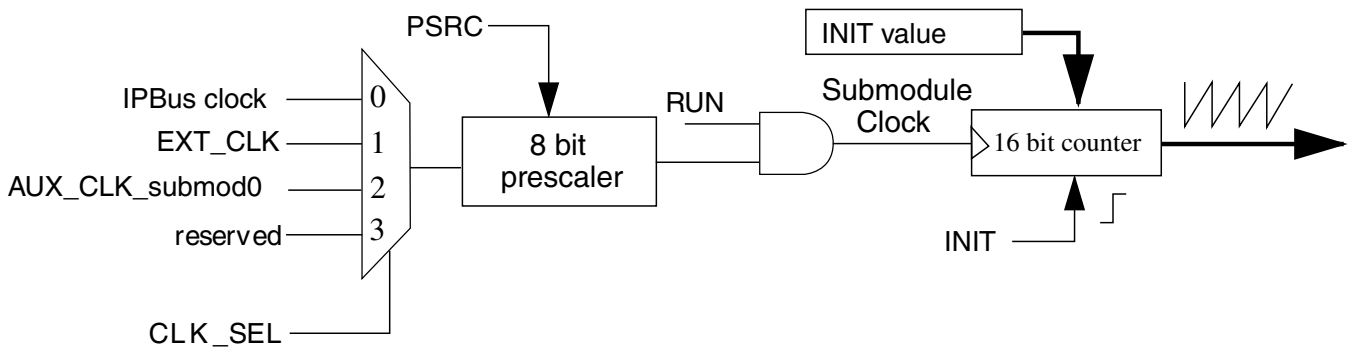
Figure 55-15. Clocking Block Diagram for PWM Submodule 1,2,3
