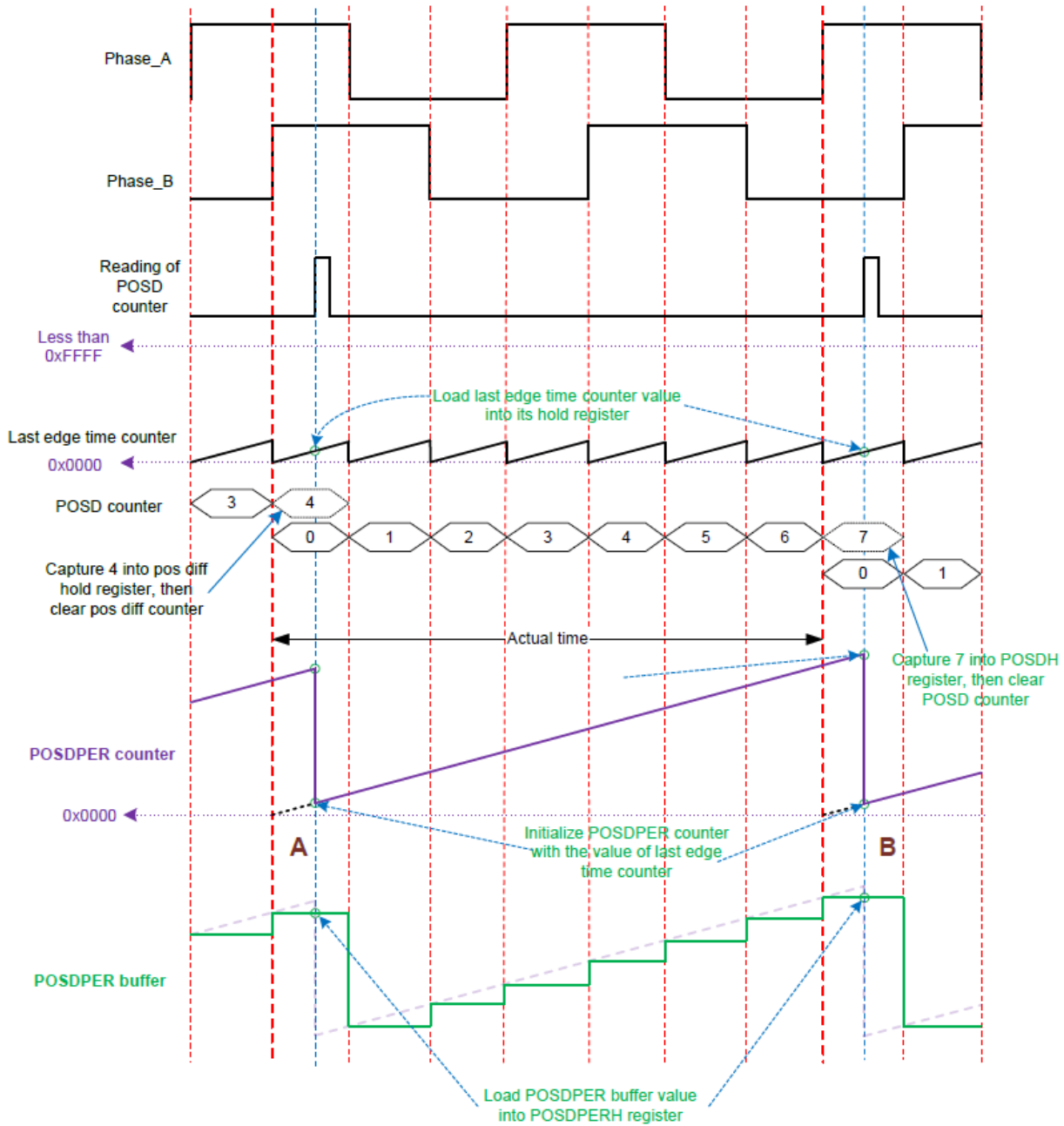
Figure 56-4. Counters behavior and updating mechanism
