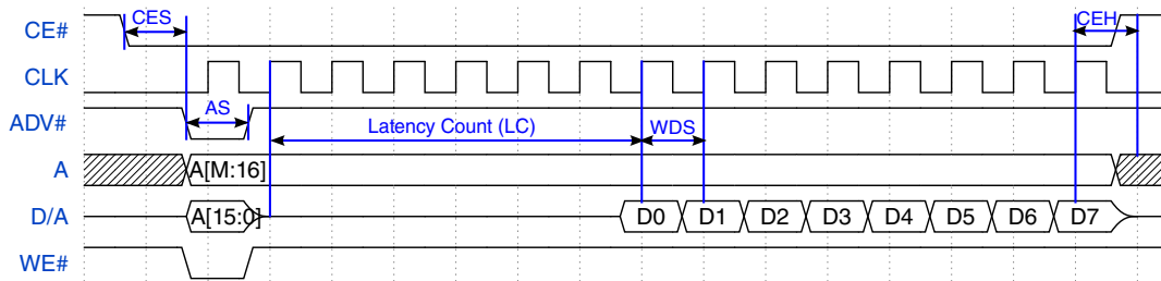
Figure 25-65. SRAM Write in SYNC Mode (ADMUX)
