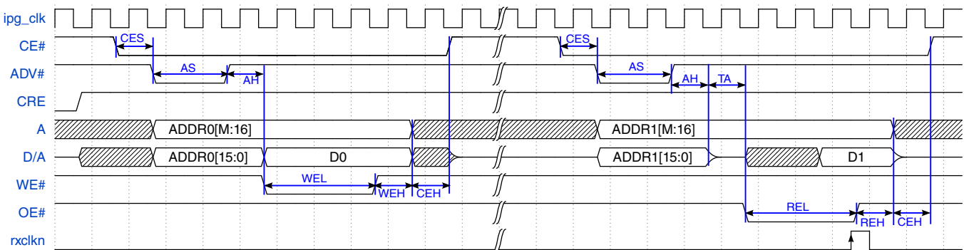
Figure 25-63. ASYNC SRAM Register Access in ADMUX Address Mode
