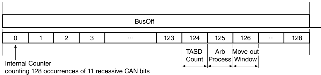
Figure 45-14. Arbitration at the end of bus off and move-out time windows
