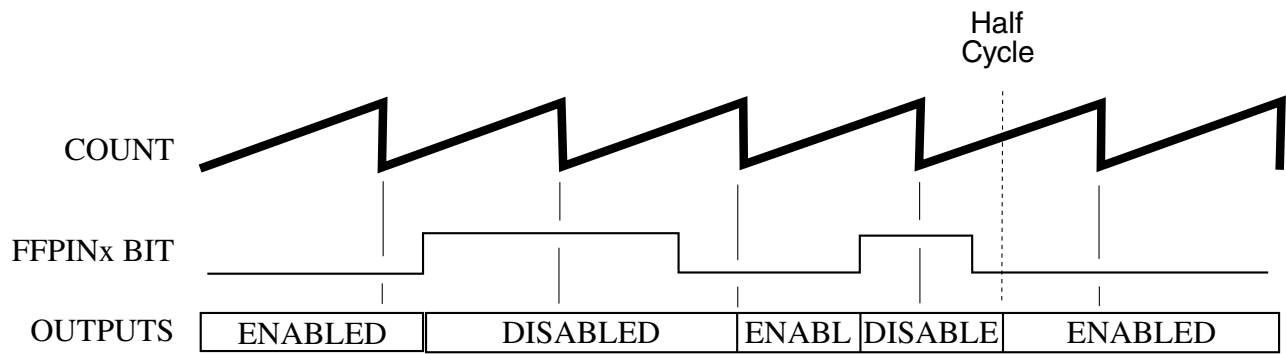
Figure 55-31. Automatic Fault Clearing
