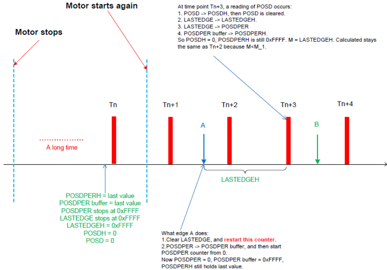
Figure 56-14. Speed measurement at time point T_{n+3}
