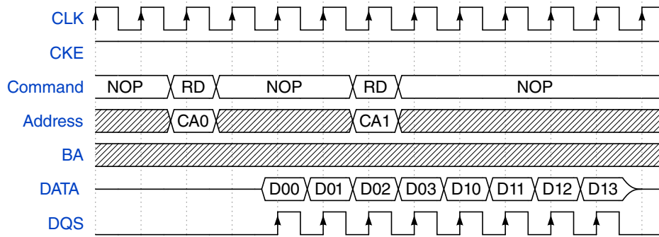
Figure 25-17. SDRAM Read-to-Read Access ( CL=2 )
