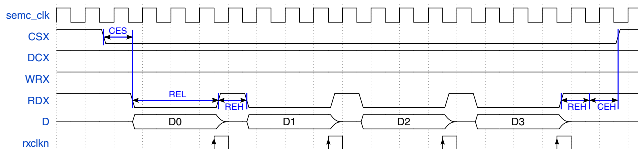
Figure 25-67. DBI Read Operation
