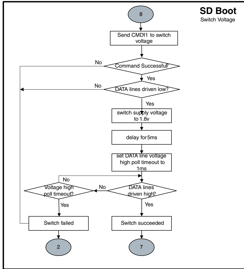
Figure 9-9. Expansion device (SD/eSD/SDXC) boot flow (3 of 6) part 2
