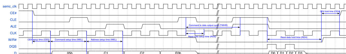
Figure 25-49. NAND Command + Address + Command + Read in SYNC Mode
