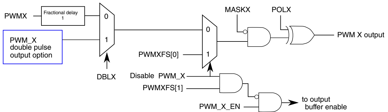
Figure 55-28. Output Logic continued
