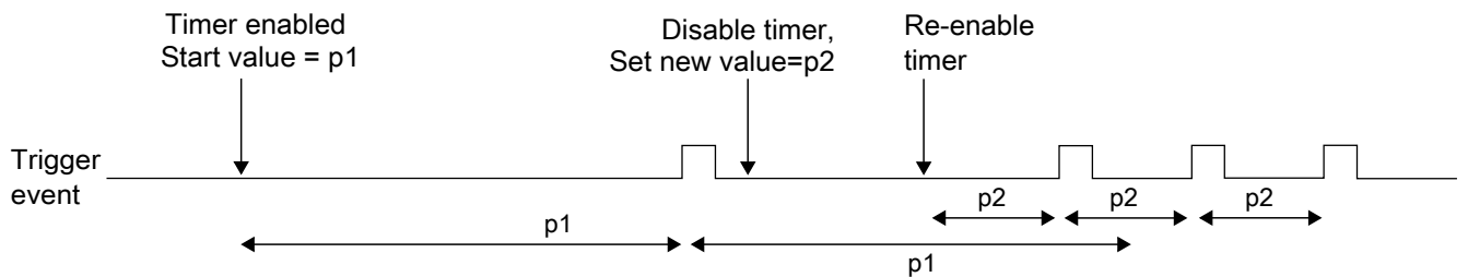
Figure 53-3. Modifying running timer period
