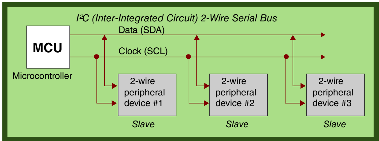
Figure 47-2. I 2 C 2-wire serial bus
