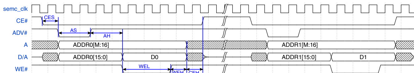
Figure 25-61. ASYNC SRAM Write in ADMUX Address Mode
