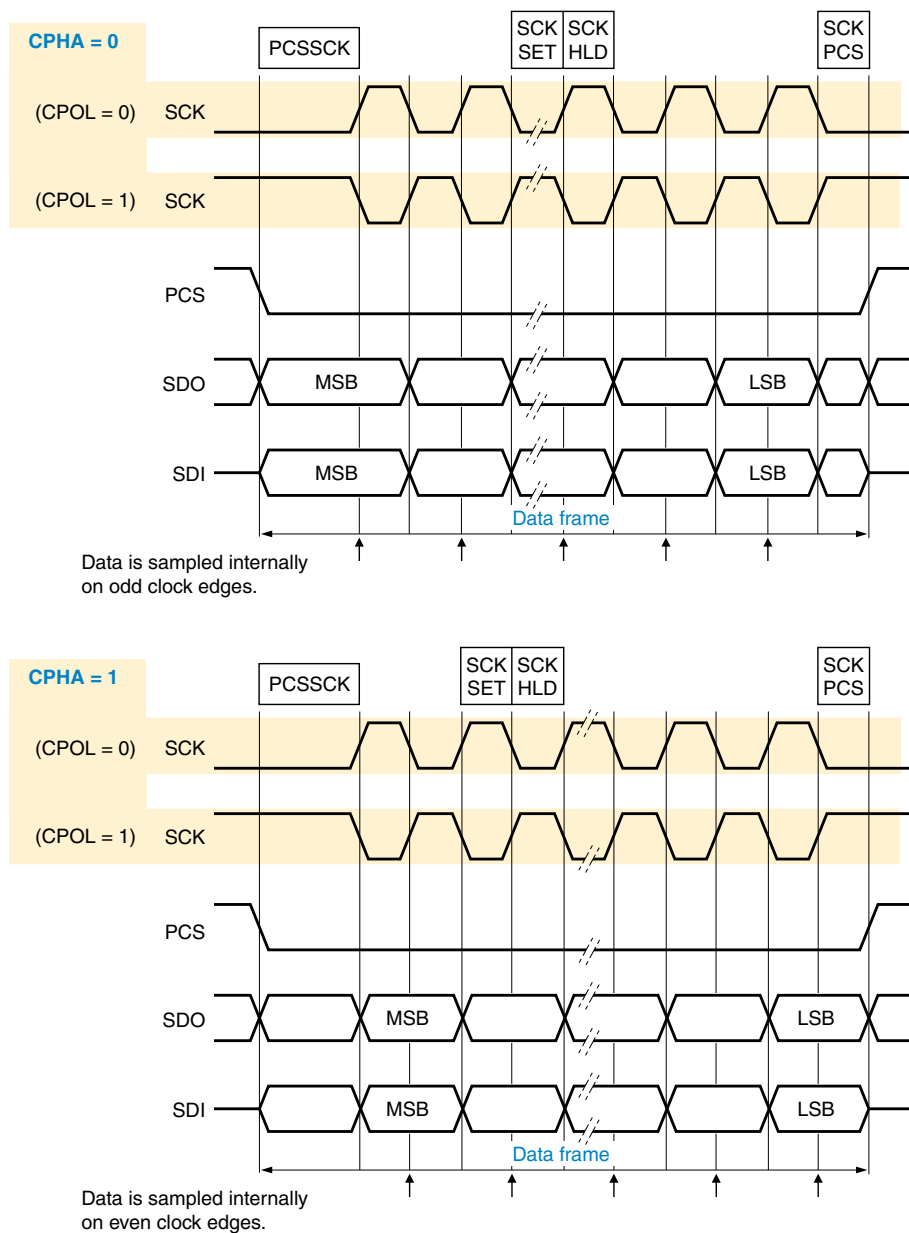
Figure 48-2. Clock Phase (TCR[CPHA]) timing diagram example
