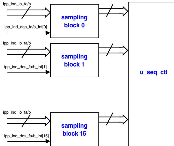
Figure 27-26. Sampling Blocks for Data Learning feature
