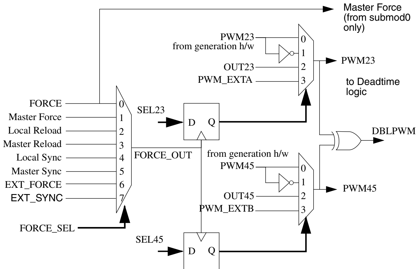
Figure 55-19. Force Out Logic
