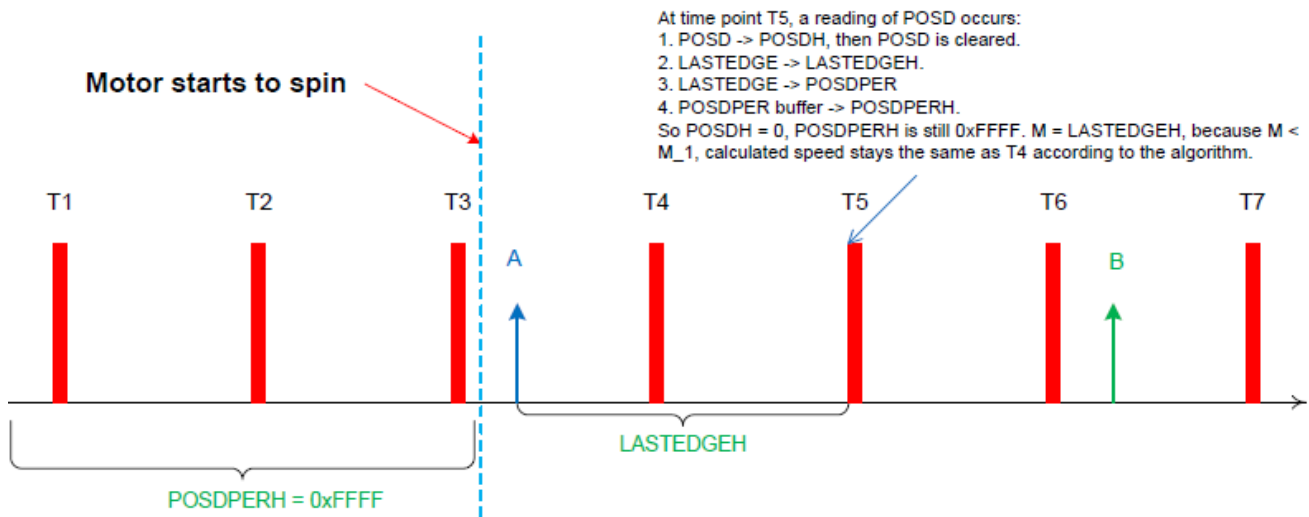
Figure 56-9. Speed measurement at time point T5
