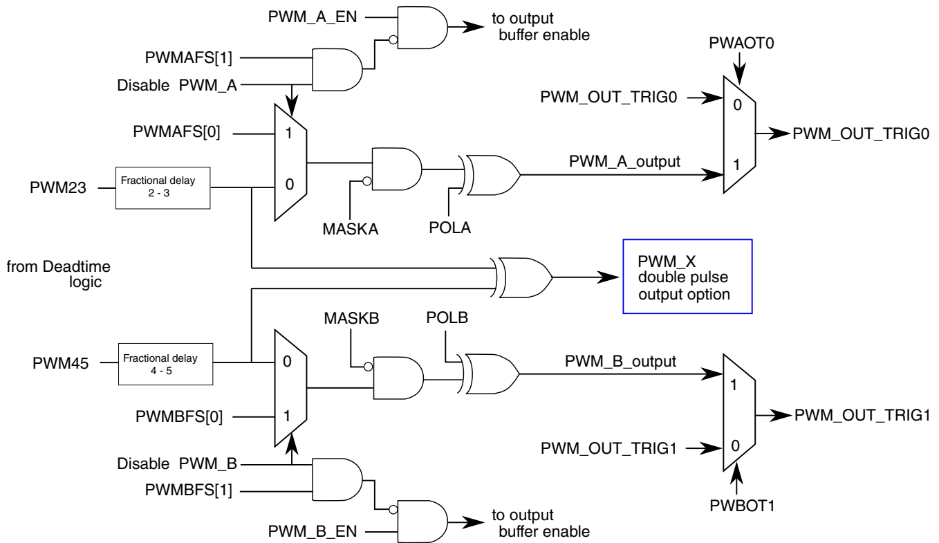
Figure 55-27. Output Logic
