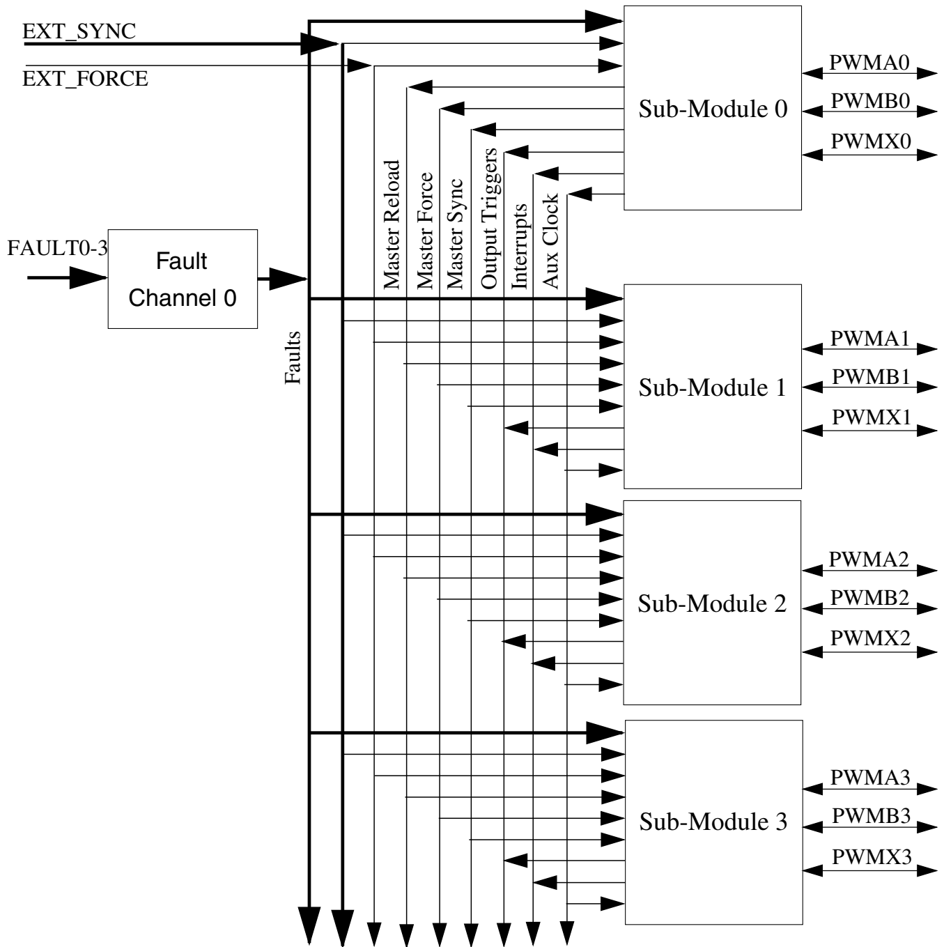
Figure 55-1. PWM Block Diagram
