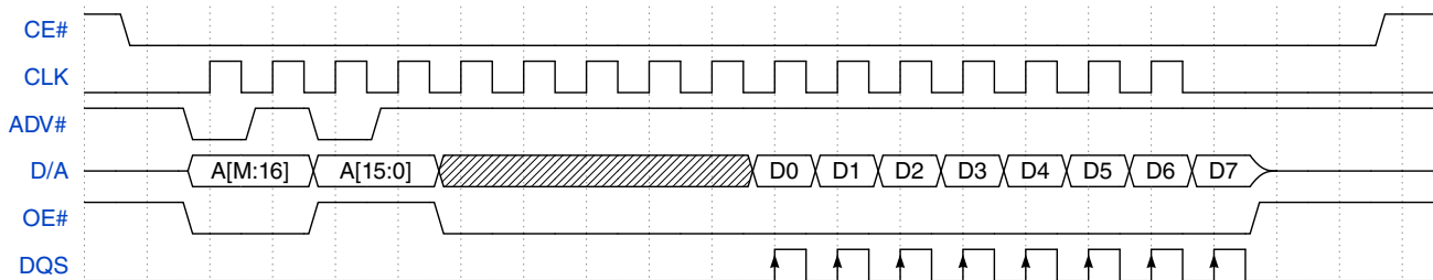
Figure 25-57. SYNC Flash Read in AADM Address Mode
