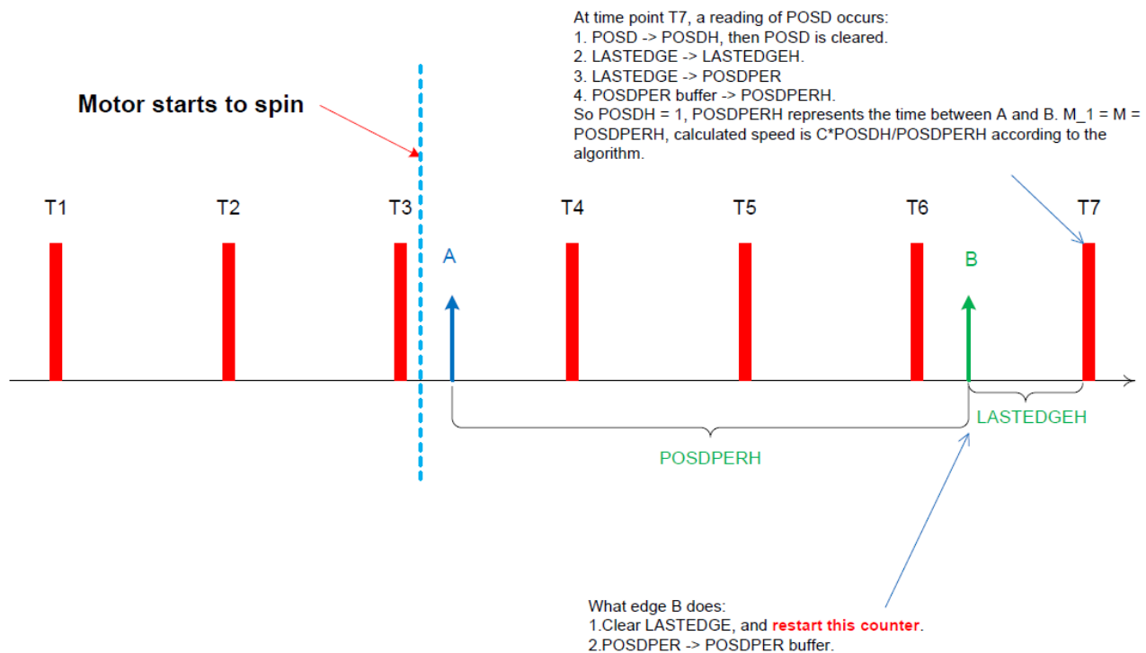
Figure 56-10. Speed measurement at time point T7
