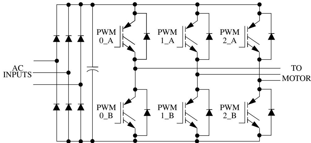
Figure 55-21. Typical 3 Phase AC Motor Drive
