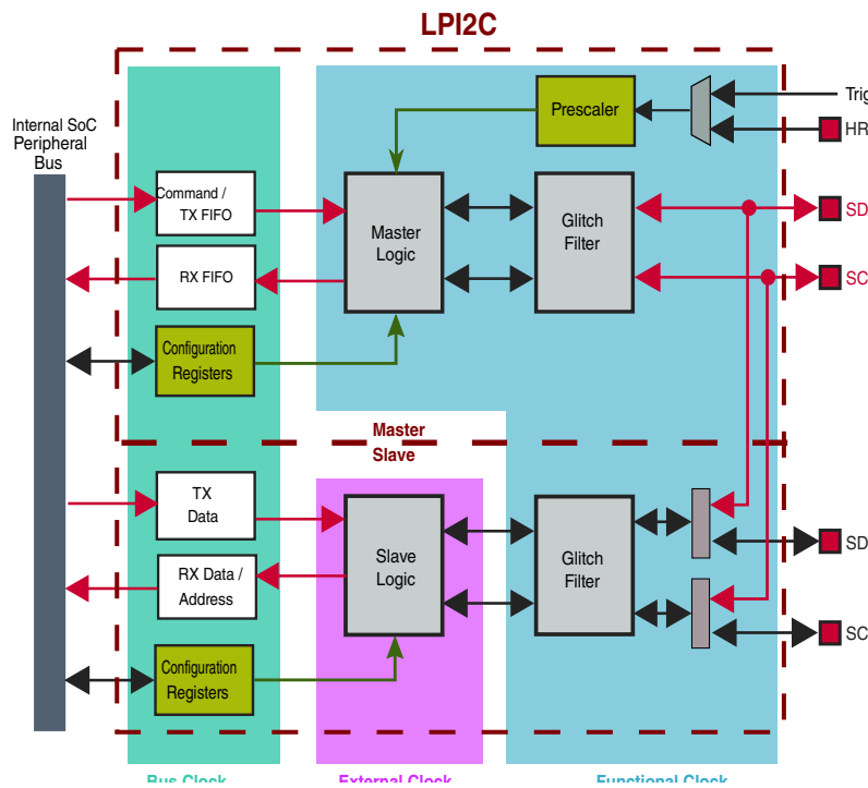
Figure 47-1. LPI2C block diagram
