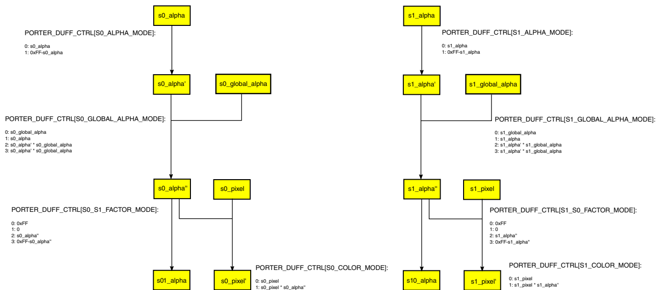
Figure 36-9. Porter-Duff Alpha Blend
