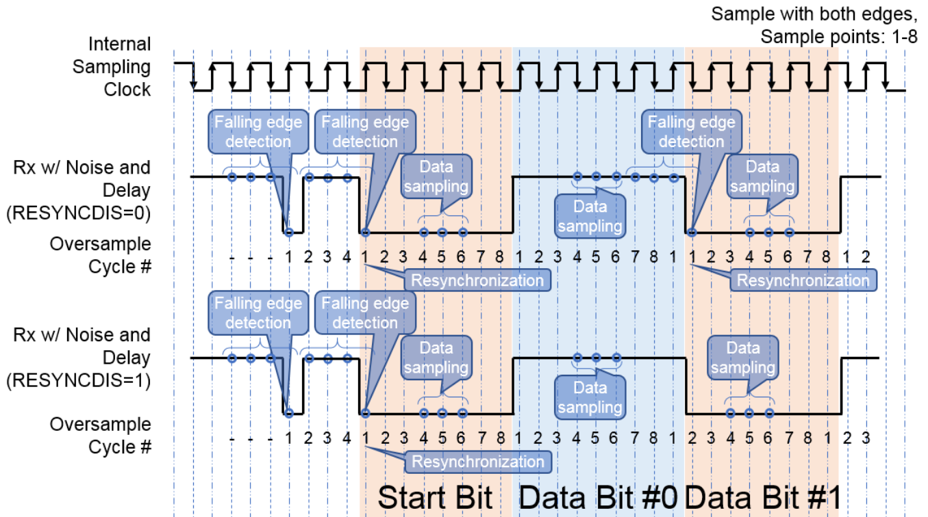
Figure 49-5. LPUART resynchronization
