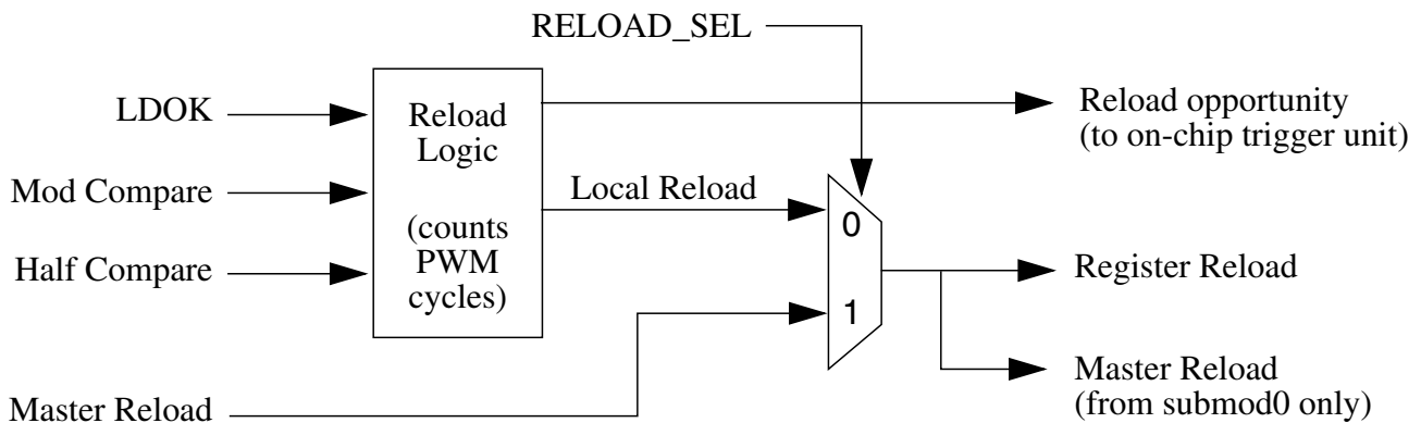
Figure 55-16. Register Reload Logic
