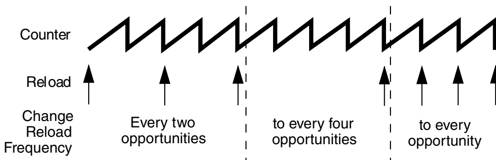
Figure 55-34. Full Cycle Reload Frequency Change
