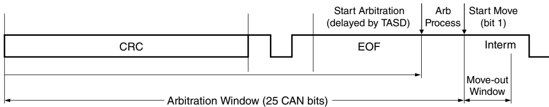
Figure 45-13. Arbitration and move-out time windows
