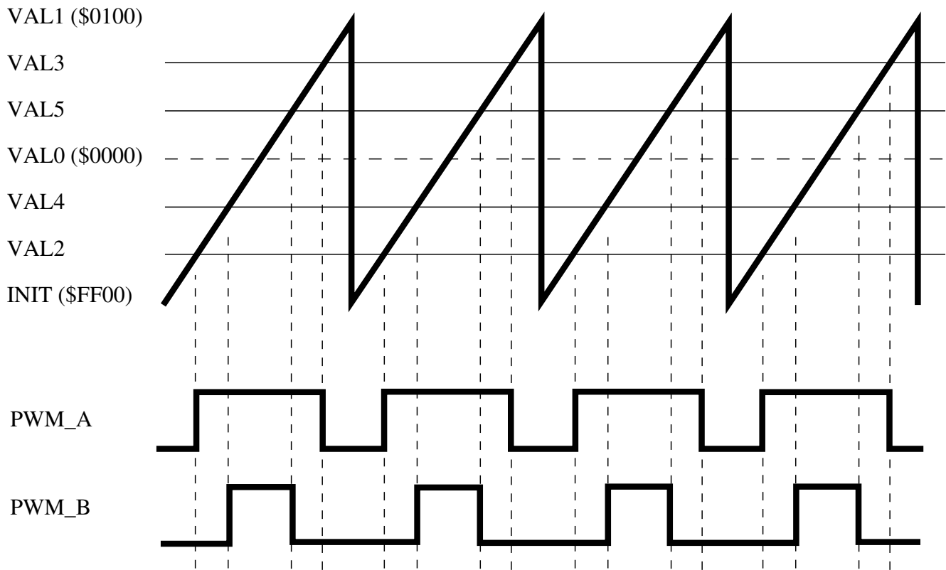
Figure 55-3. Center Aligned Example
