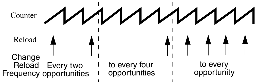
Figure 55-35. Half Cycle Reload Frequency Change
