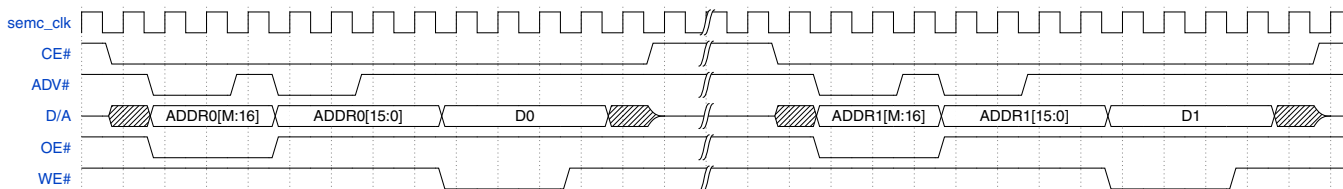
Figure 25-55. ASYNC NOR Flash Write in AADM Address Mode
