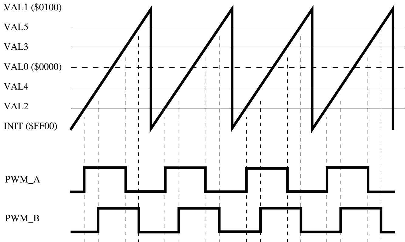
Figure 55-5. Phase Shifted Outputs Example
