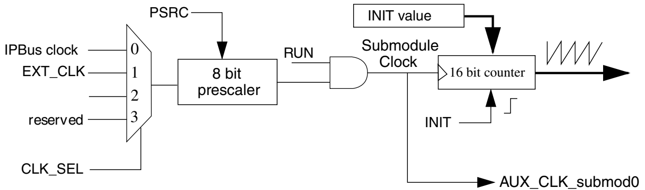
Figure 55-14. Clocking Block Diagram for PWM Submodule 0
