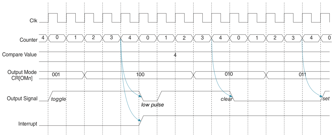
Figure 52-5. Output Compare and Interrupt Timing
