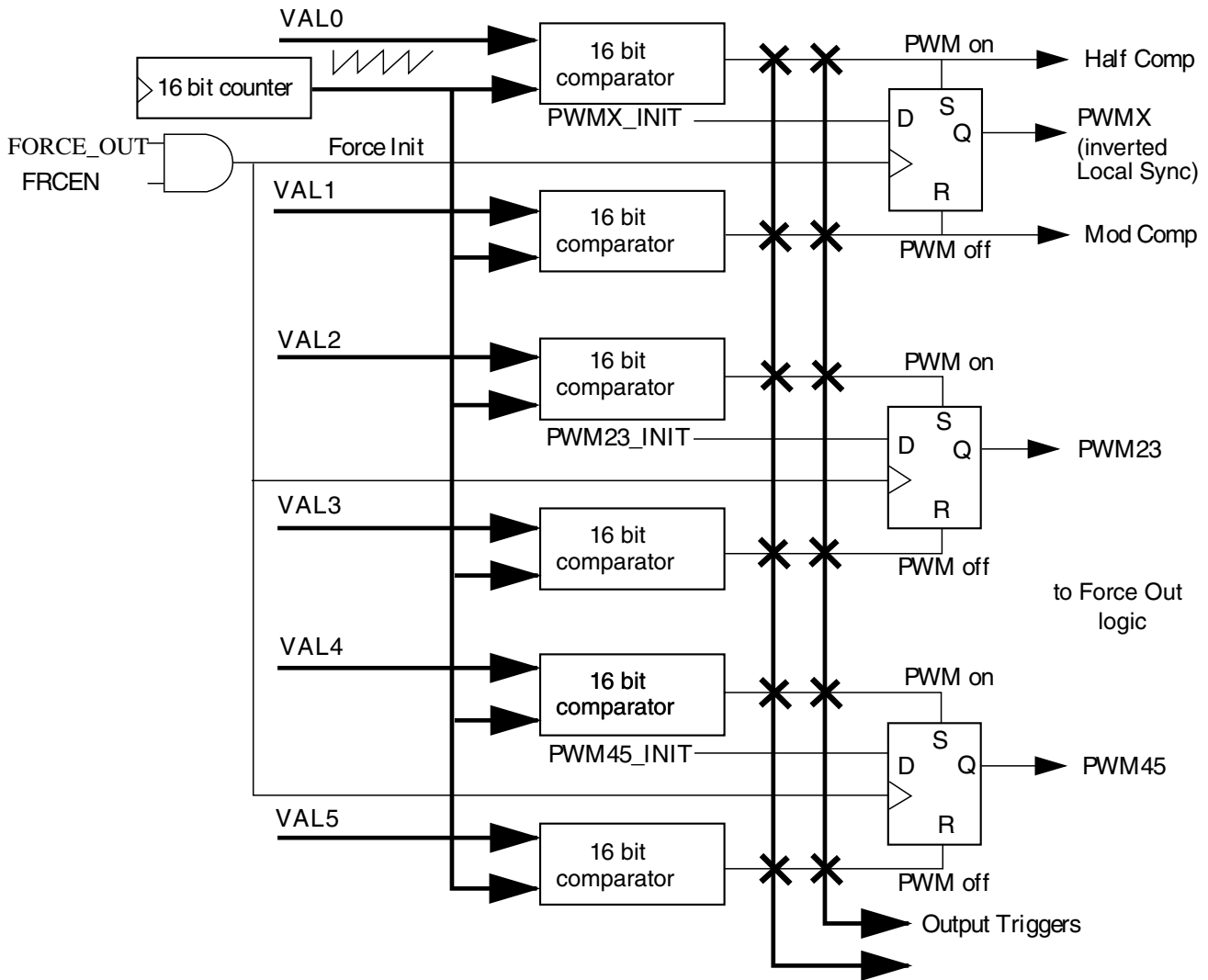
Figure 55-18. PWM Generation Hardware
