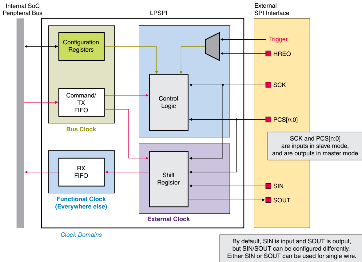
Figure 48-1. Block diagram
