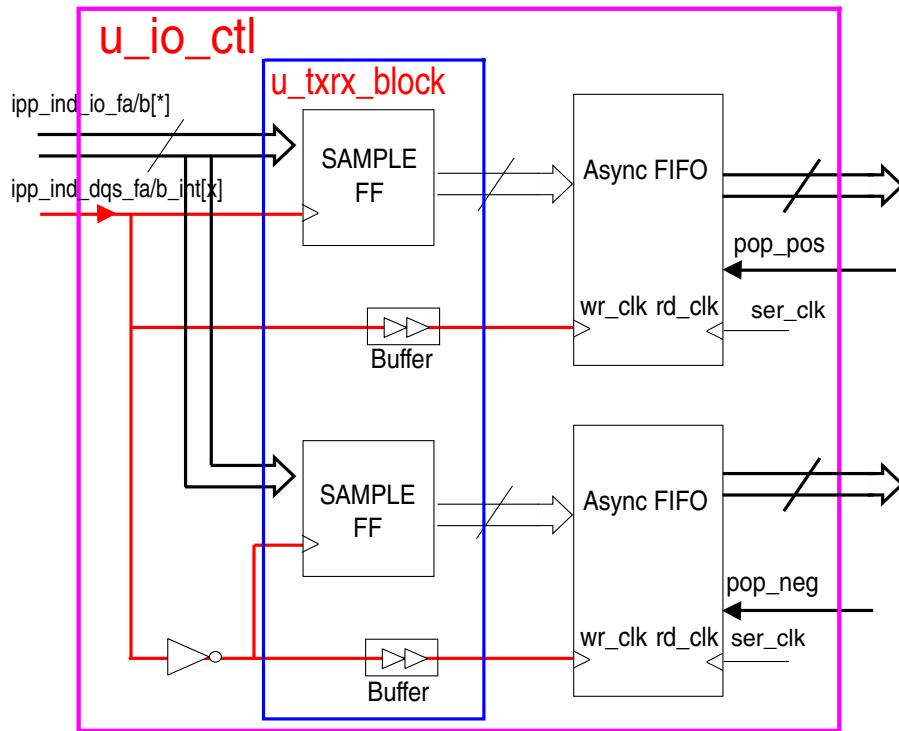
Figure 27-25. Sampling Block in FlexSPI
