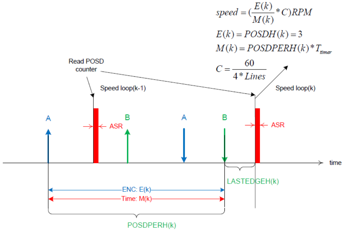
Figure 56-5. High speed measurement with method
