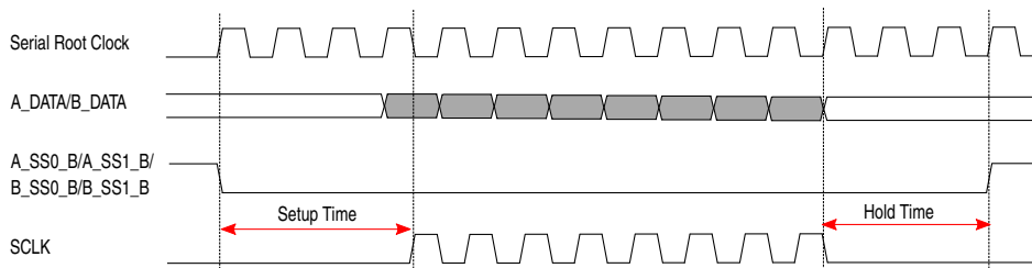
Figure 27-22. Chip selection output timing for SDR sequence
