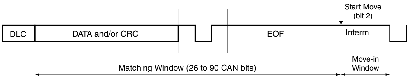
Figure 45-12. Matching and move-in time windows
