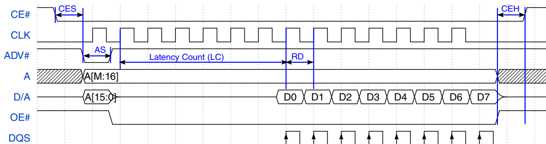
Figure 25-64. SYNC SRAM Read in ADMUX Address Mode
