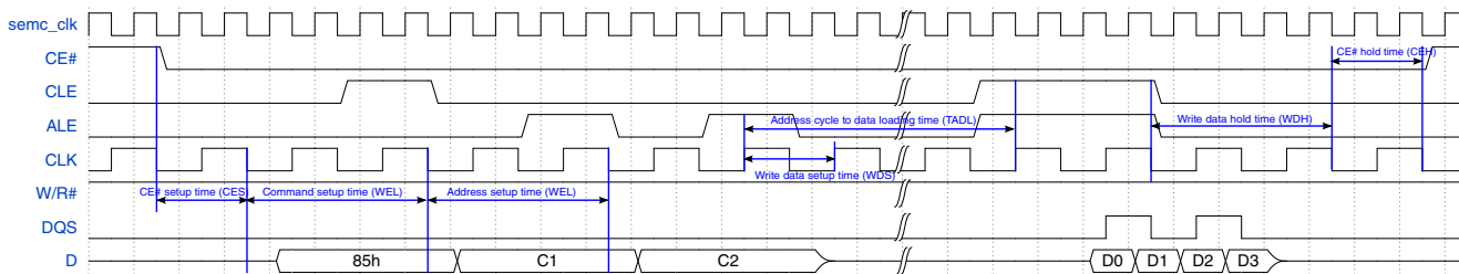
Figure 25-50. NAND Command + Address + Write in SYNC Mode
