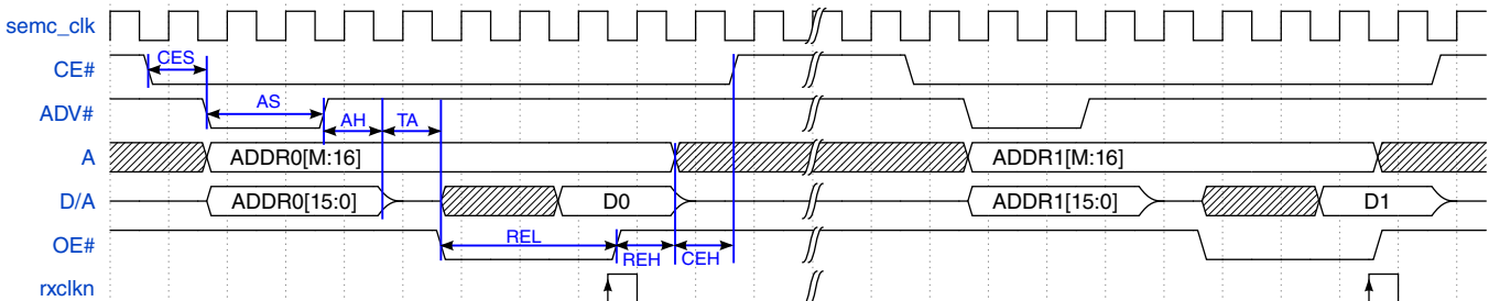
Figure 25-59. ASYNC SRAM Read in ADMUX Address Mode
