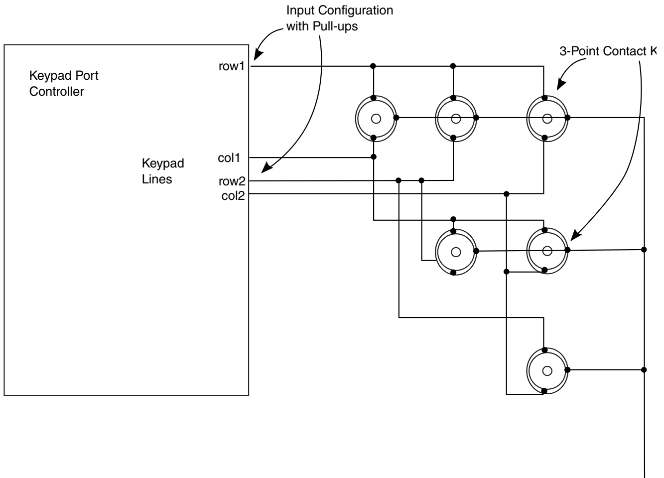
Figure 46-7. KPP Interface with 3-point Contact Key Matrix (Simplified View)
