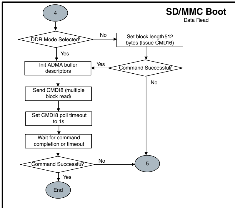
Figure 9-11. Expansion device (SD/eSD) boot flow (5 of 6)
