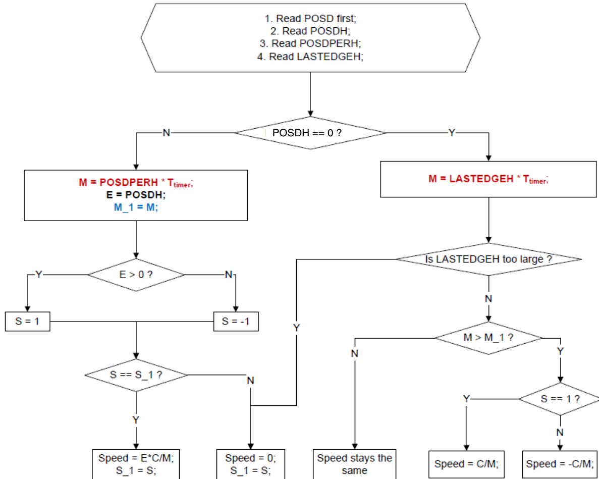
Figure 56-6. Flowchart of speed calculation with method
