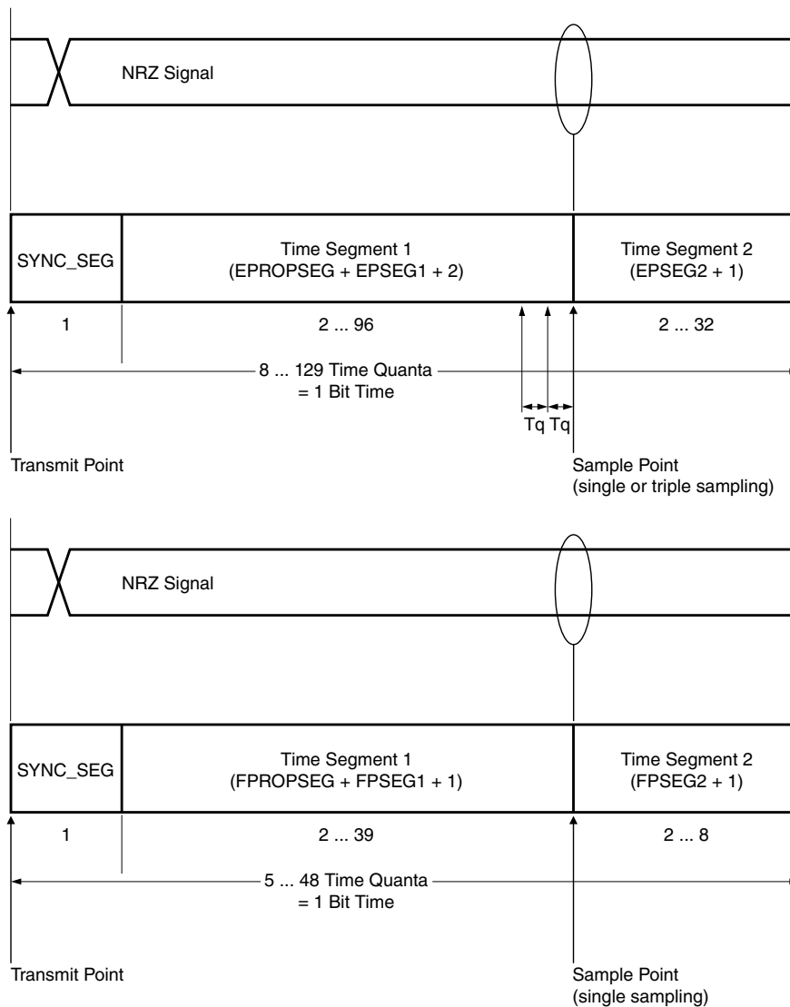
Figure 45-10. Segments within the bit time (example using CBT and FDCBT bit timing variables for CAN FD format)
