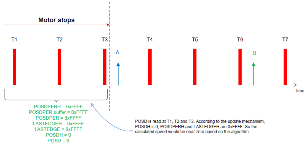
Figure 56-7. Speed measurement at time point T1~T3
