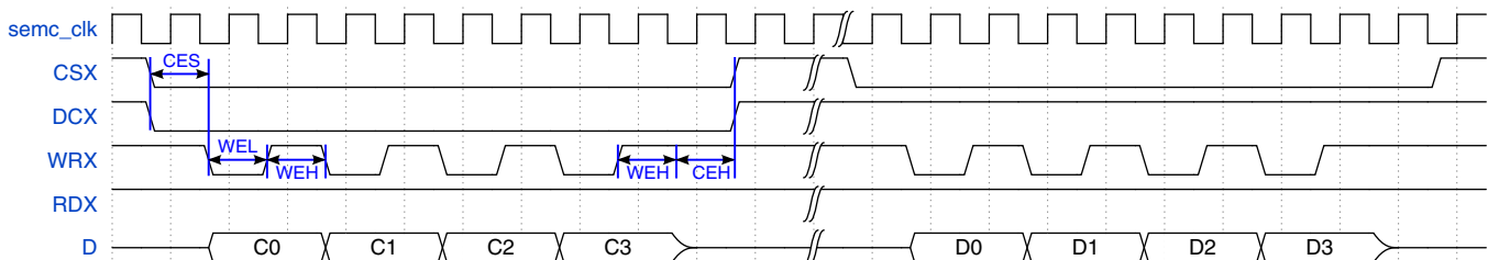
Figure 25-66. DBI Write Operation
