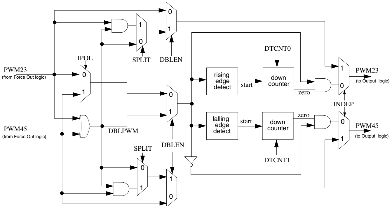
Figure 55-22. Deadtime Insertion Logic
