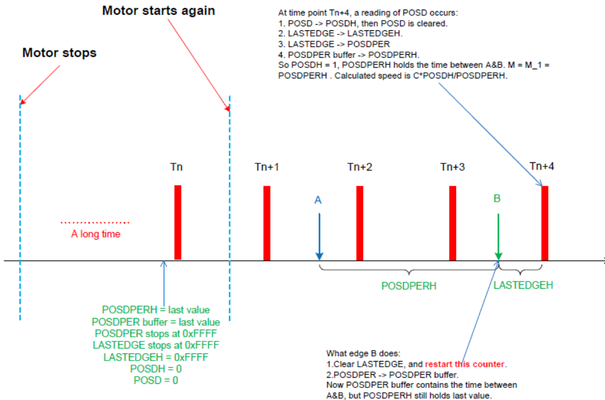
Figure 56-15. Speed measurement at time point Tn+4
