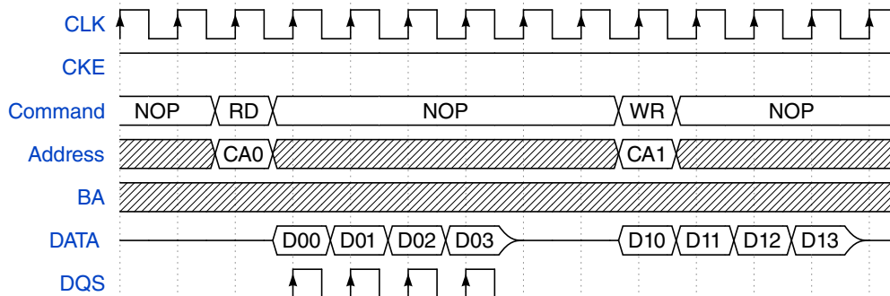
Figure 25-19. SDRAM Read-to-Write Access ( CL=1 )
