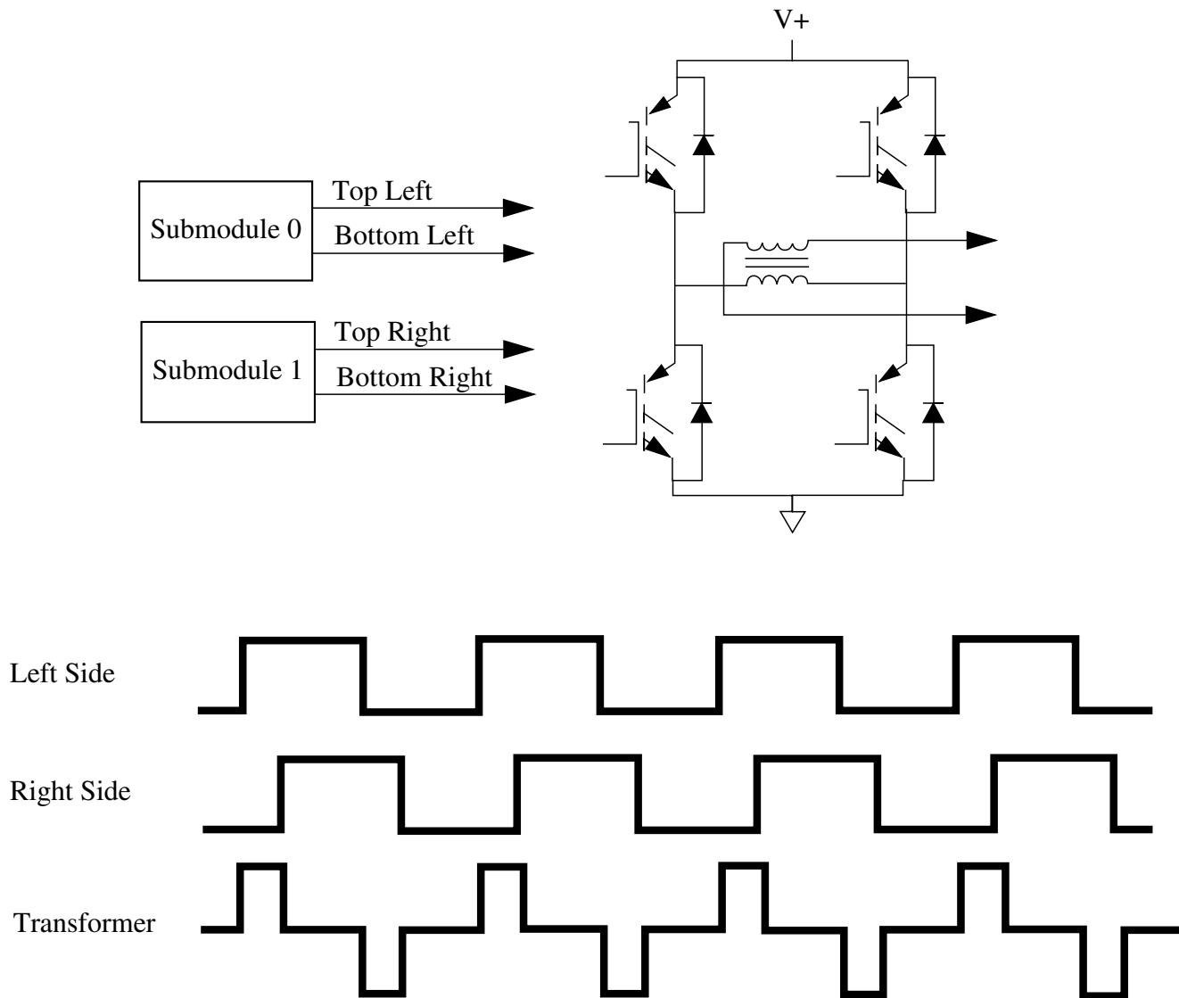
Figure 55-6. Phase Shifted PWMs Applied to a Transformer Primary
