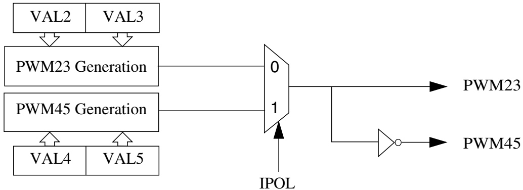
Figure 55-20. Complementary Channel Pair
