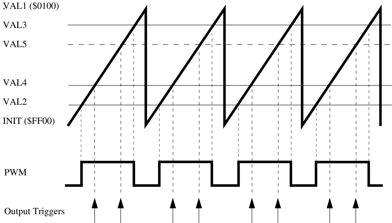
Figure 55-8. Multiple Output Trigger Generation in Hardware
