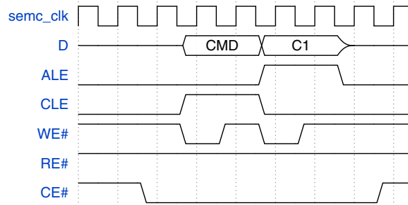
Figure 25-30. NAND Flash Access Address Type - One Byte Column Address
