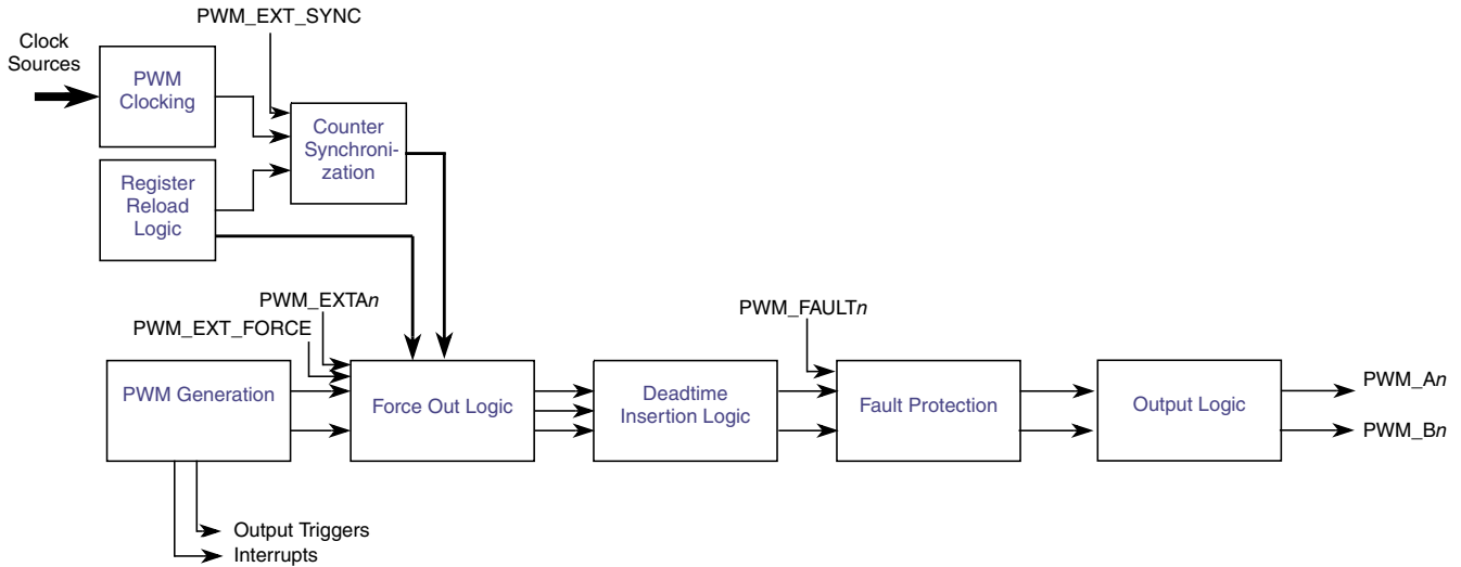
Figure 55-13. High-Level Output PWM Generation Block Diagram
