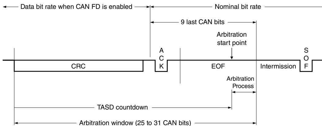
Figure 45-15. Optimal Tx Arbitration start point
