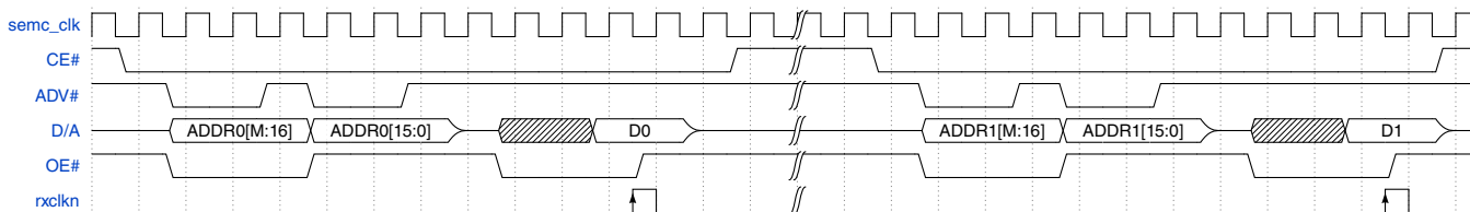
Figure 25-53. ASYNC NOR Flash Read in AADM Address Mode
