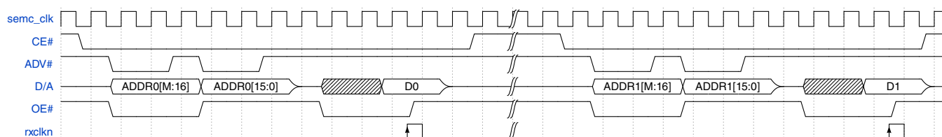
Figure 25-60. ASYNC SRAM Read in AADM Address Mode
