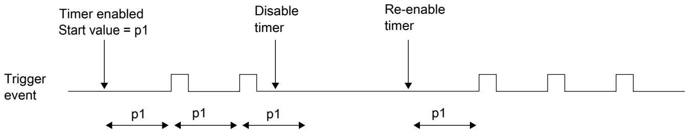
Figure 53-2. Stopping and starting a timer
