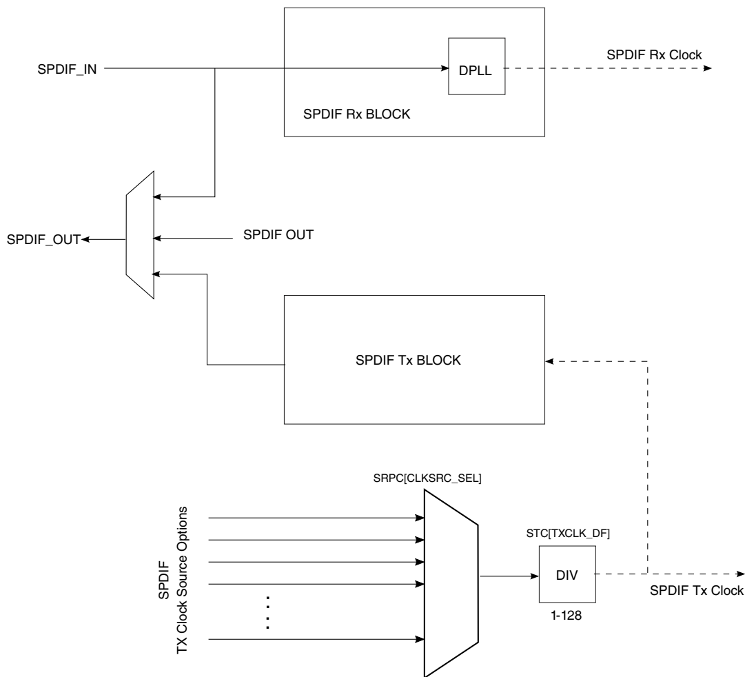
Figure 40-2. SPDIF Transceiver Clock Diagram
