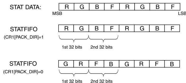
Figure 34-9. Data Packing
