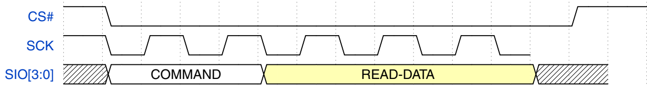
Figure 27-27. Unsupported Read Behavior
