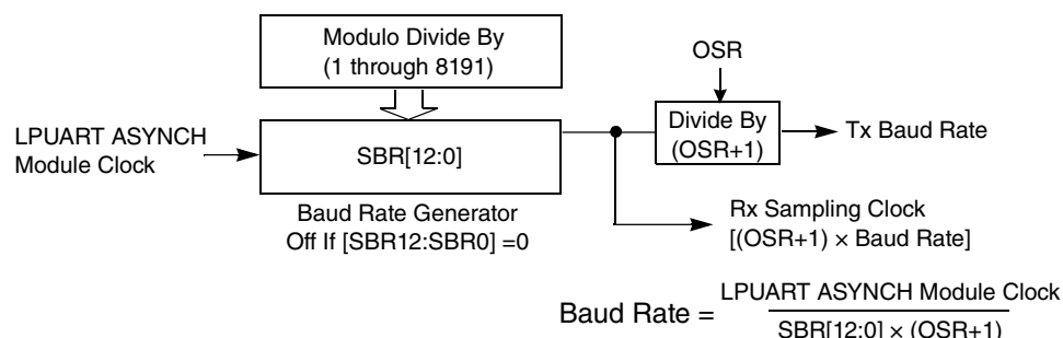
Figure 49-3. LPUART baud rate generation
