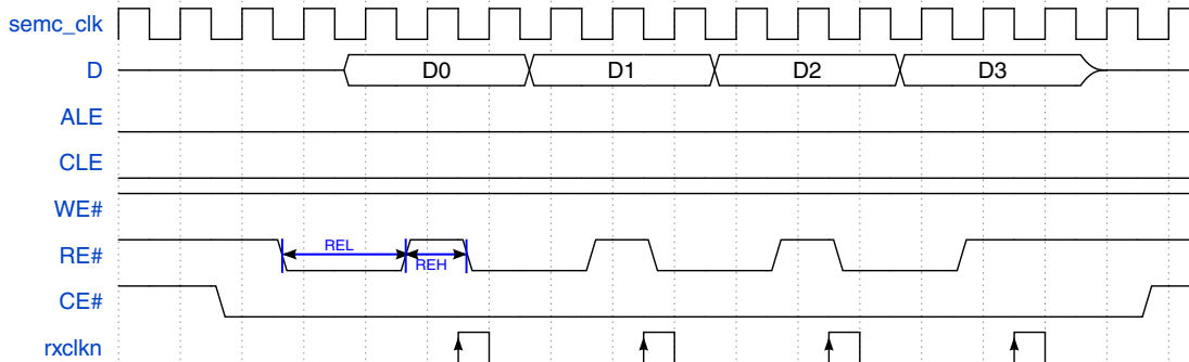
Figure 25-47. NAND Flash Read Access in EDO mode
