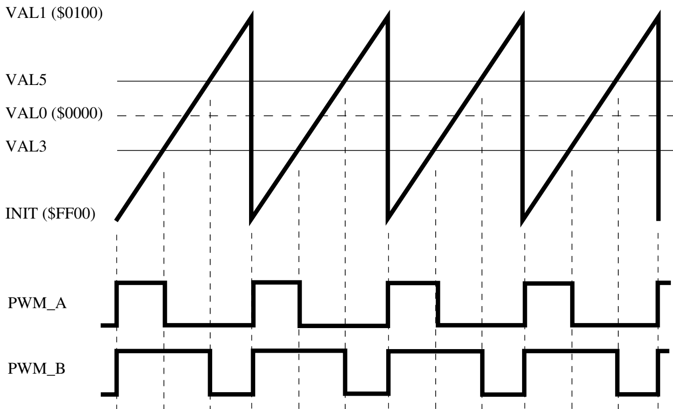
Figure 55-4. Edge Aligned Example (INIT=VAL2=VAL4)
