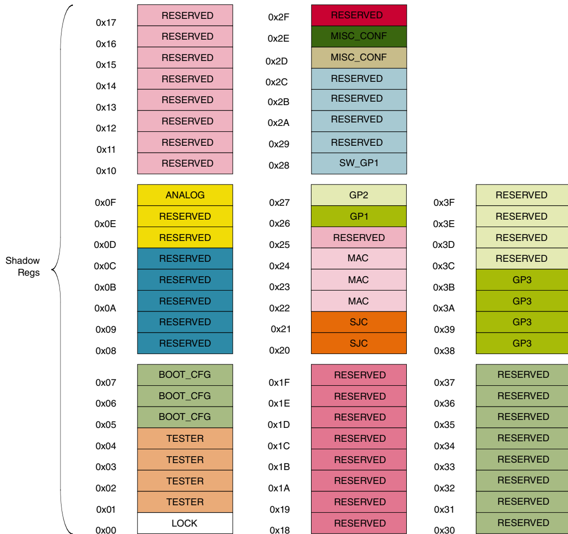
Figure 23-2. OTP Memory Footprint
