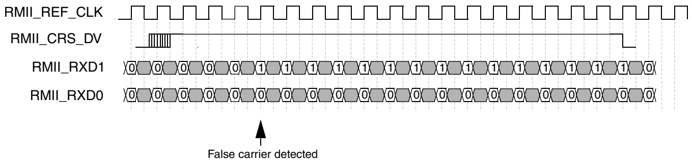
Figure 41-20. RMII receive operation with false carrier
