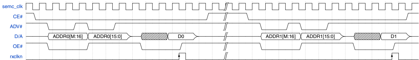
Figure 25-60. ASYNC SRAM Read in AADM Address Mode
