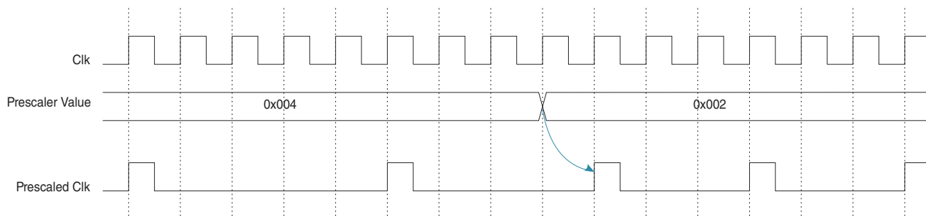
Figure 52-3. Prescaler Value Change Timing Diagram
