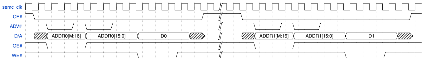
Figure 25-55. ASYNC NOR Flash Write in AADM Address Mode
