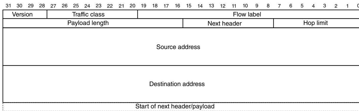
Figure 41-4. IPv6 header format
