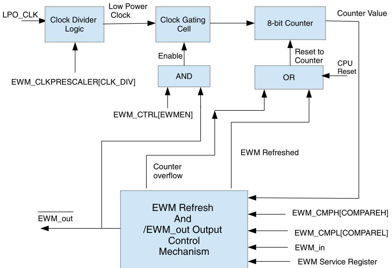
Figure 59-1. EWM Block Diagram
