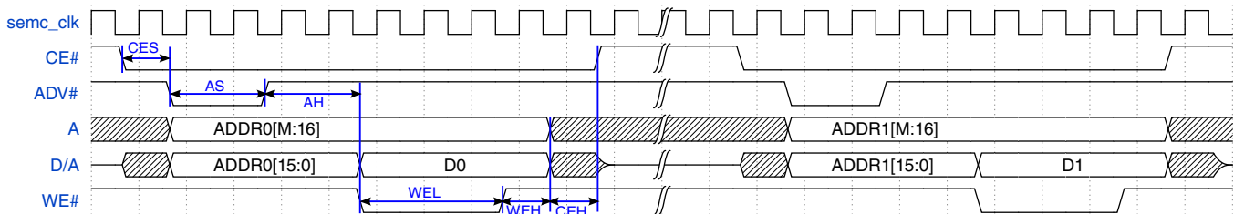
Figure 25-61. ASYNC SRAM Write in ADMUX Address Mode
